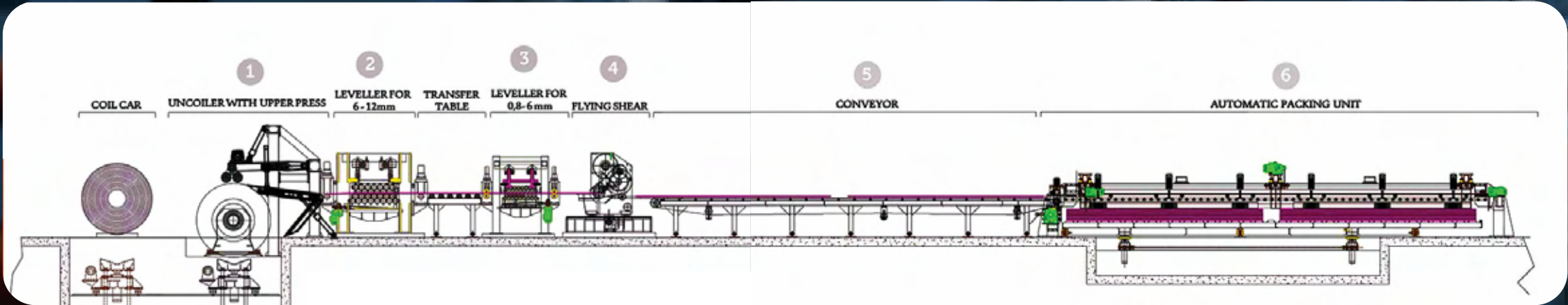
Cut to Length – 1 to 12 mm Thickness
