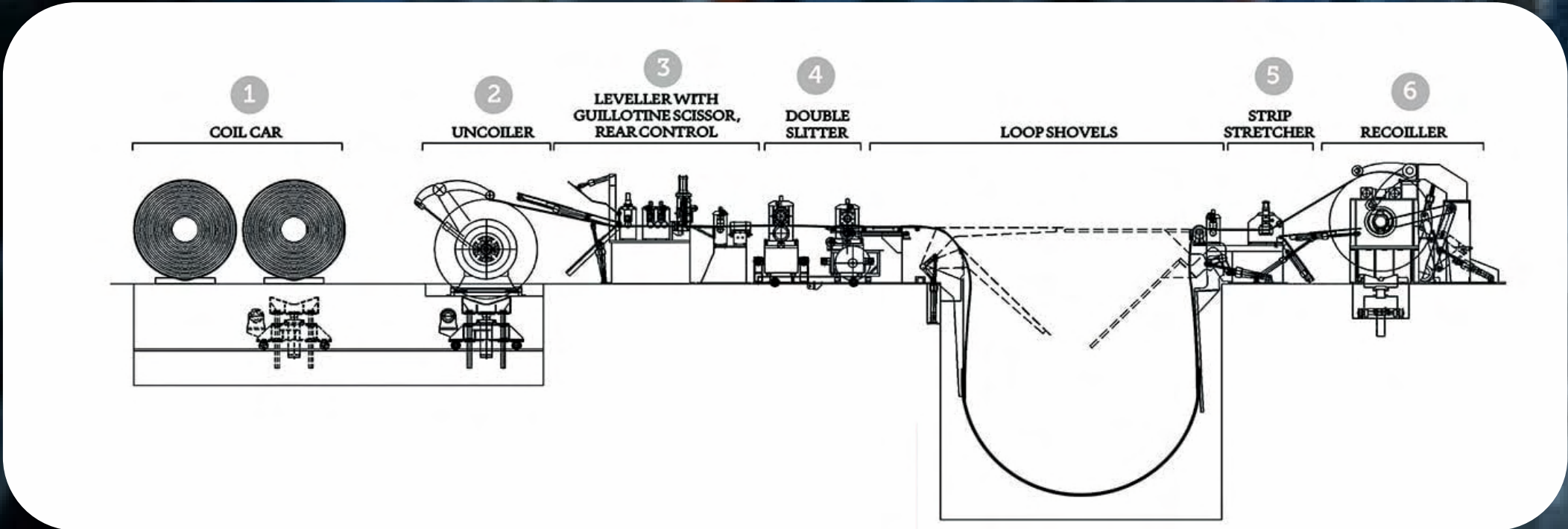
Steel Slitting – 1 to 7 mm Thickness
